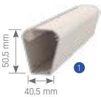
Fabric Profile
