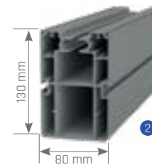
Rails
