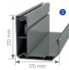
Extruded Frontal Gutter (Water-drain)
