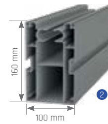
Rails
