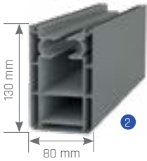
Rails
